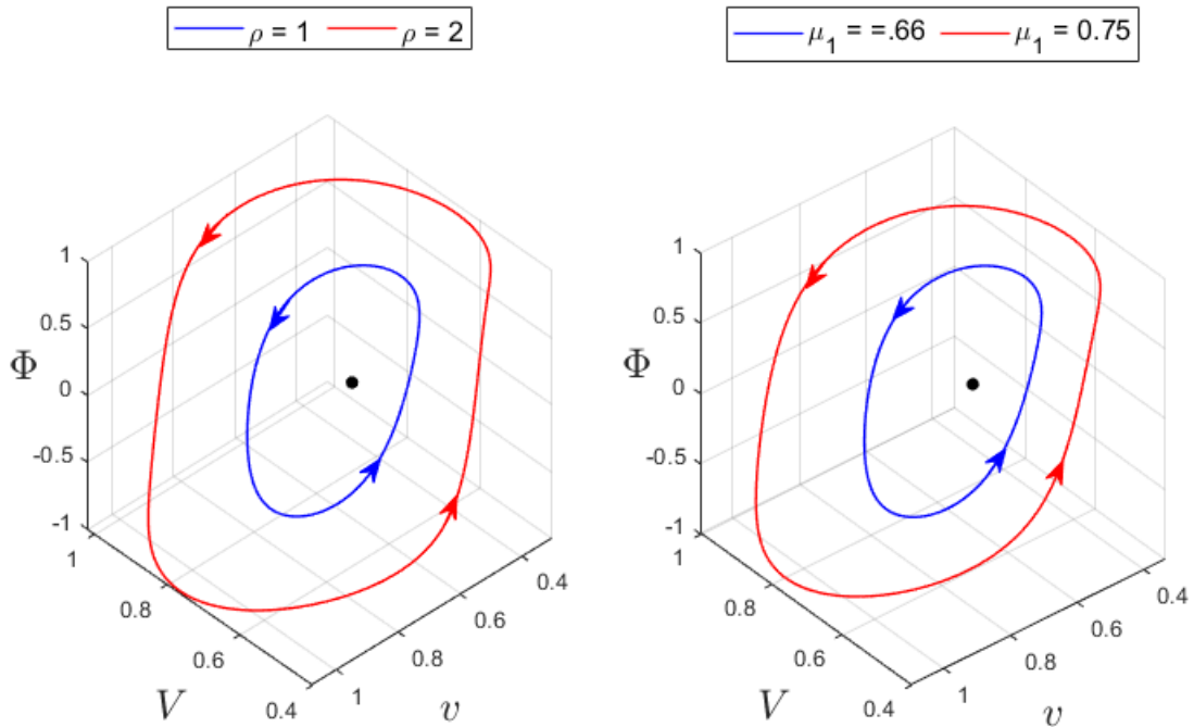
Figure 8: Robustness of closed orbits to changes in attitudes' response to employment and to variations in the response of energy efficiency to taxing emissions. The black dot stands for the equilibrium point.
