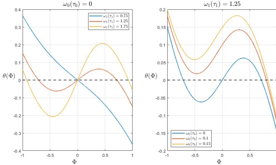
Figure 4: Emergence and control of multi-stability. The intersections between the blue, orange and yellow colours with the black dotted line correspond to the equilibrium points. The left panel shows that raising \omega_1 leads to two additional equilibria. The right panel indicates increasing \omega_0 can restore a unique equilibrium solution.
