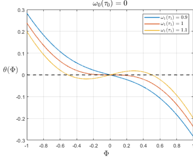
Figure A.1: Emergence of multiple equilibrium points when \tau_0 = 0 .
